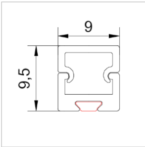
Magnet fixing Type A
