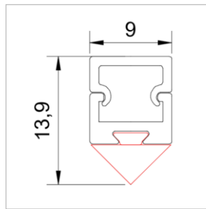
Magnet fixing Type B
